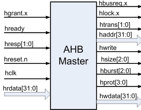
Figure 1. The AHB master interface diagram
