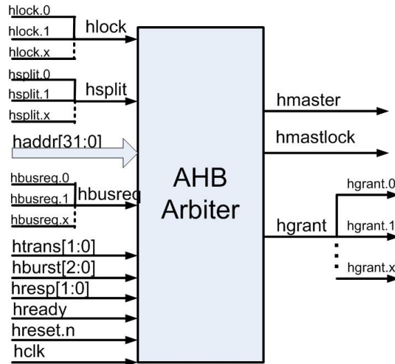
Figure 3. The AHB arbiter interface diagram
