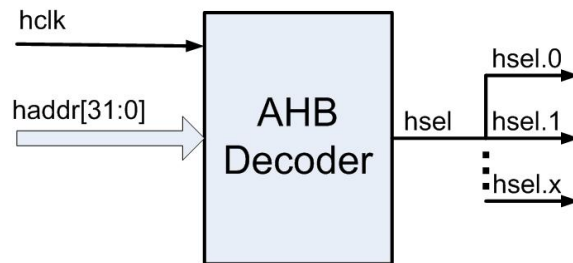
Figure 4. The AHB decoder interface diagram
