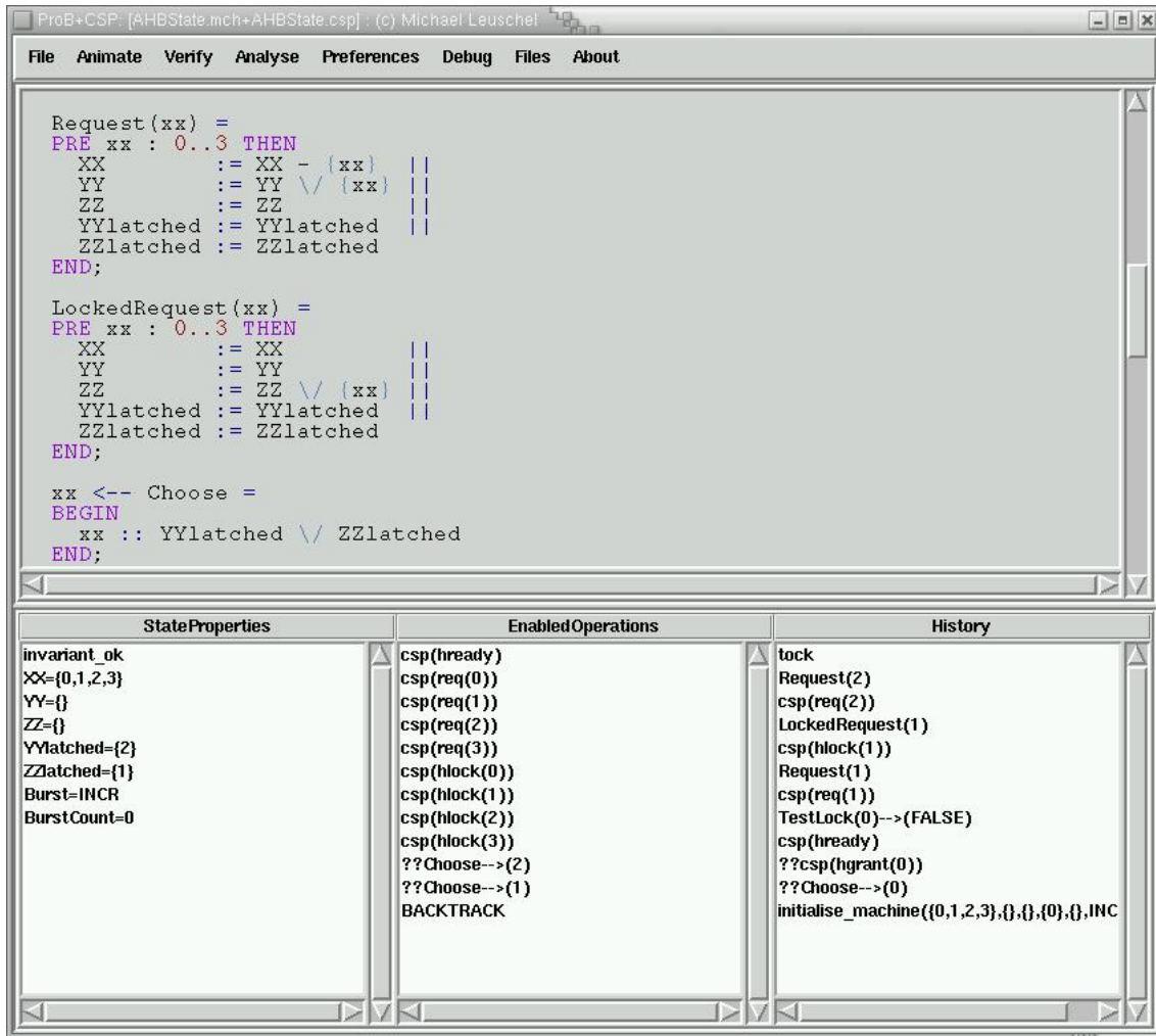
Figure 6. A snapshot of animating the model (with 4 masters) in ProB
