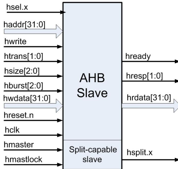
Figure 2. The AHB slave interface diagram
